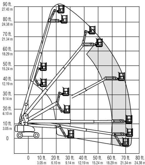
80'+6' Straight Boom
