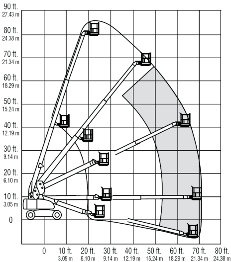
80' Straight Boom
